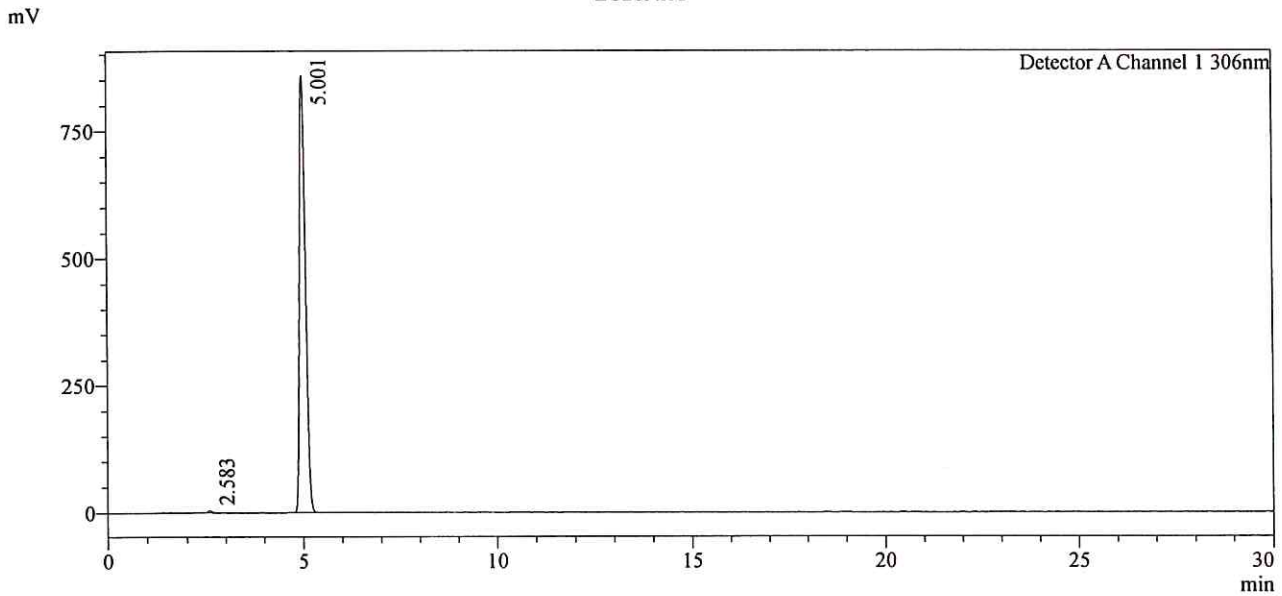
Chromatogram EC269.lcd
